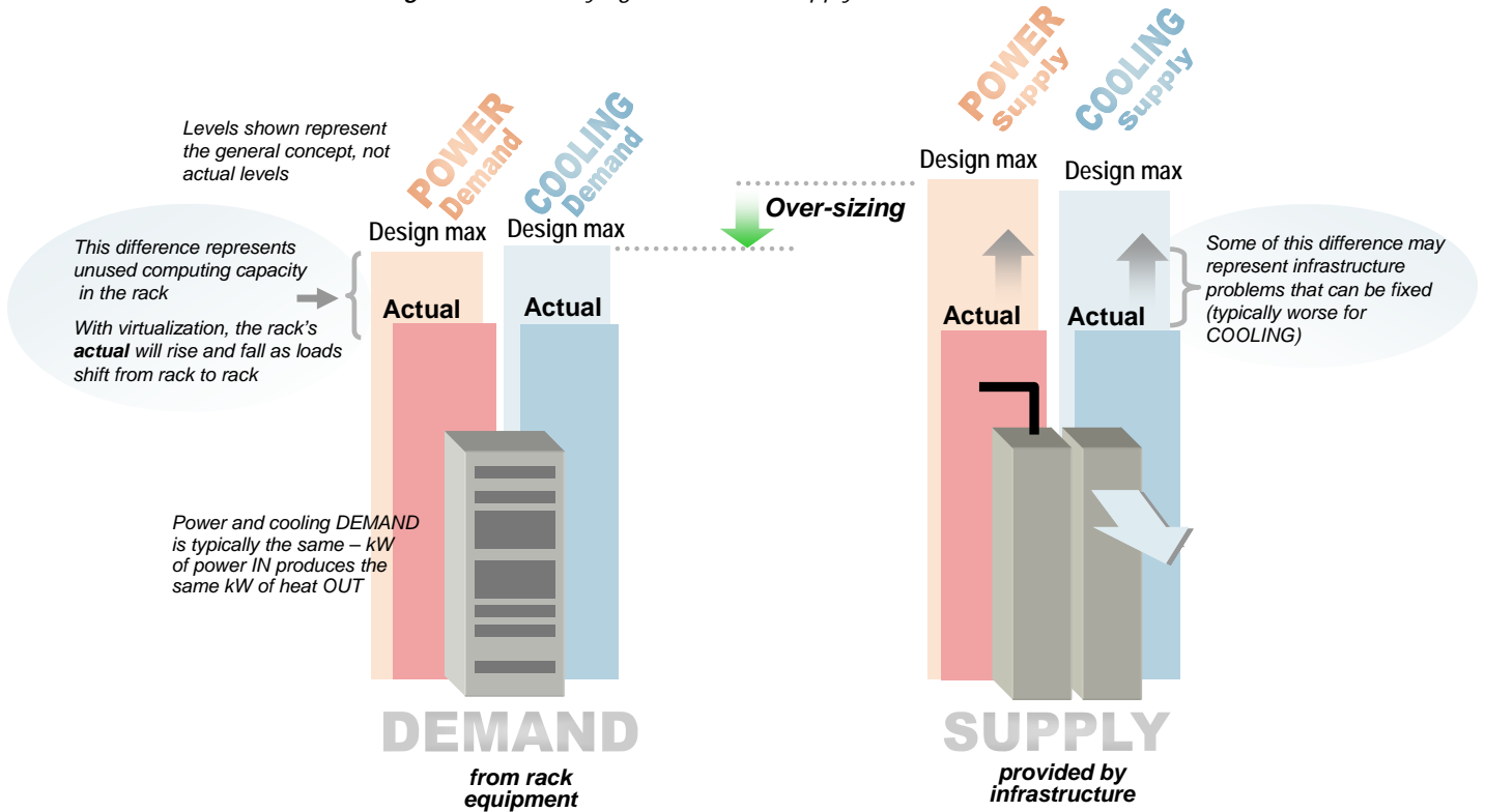
Figure 3 – Quantifying demand and supply at the rack level
